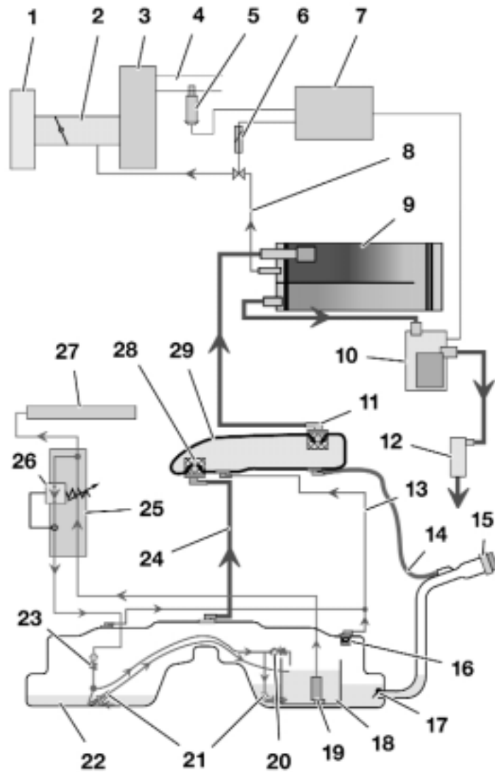
Fuel System
